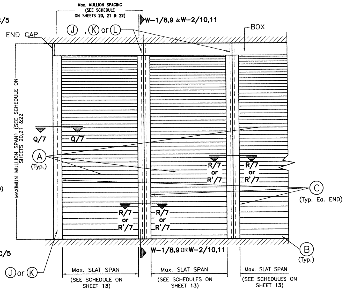
TYPICAL CONSECUTIVE SINGLE UNIT ELEVATION W/ MULLION INTO POURED CONCRETE NOTE: SEE SHEETS 2 & 3 FOR COMPONENTS NOMENCLATURE. N.T.S.
