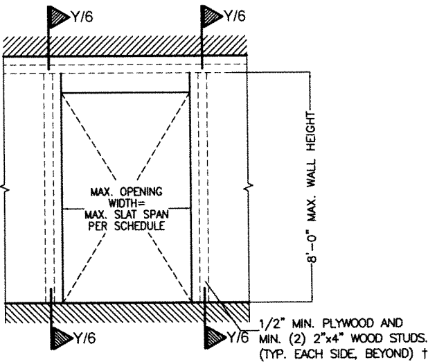
DETAIL 1 (ELEVATION)
